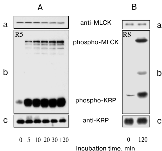
Fig. 4. Selectivity of phosphospecific antibodies against MLCK and KRP in smooth muscle tissue extracts. Rat ileum extracts were incubated at 30^{\circ}\text{C} with 4 mM \text{Mg}^{2+} -ATP (pH 7.4) and either PKA (A) or activated GST-p44 erk1 -MAP-kinase (B). Equal aliquots of the reaction mixtures were withdrawn at indicated time intervals and analyzed by immunoblotting. The total amount of MLCK (a) and KRP (c) was determined by the polyclonal anti-KRP antibody staining. Phosphorylated MLCK and KRP were analyzed with phosphospecific R5 (A) or R8 (B) antibodies (b).
