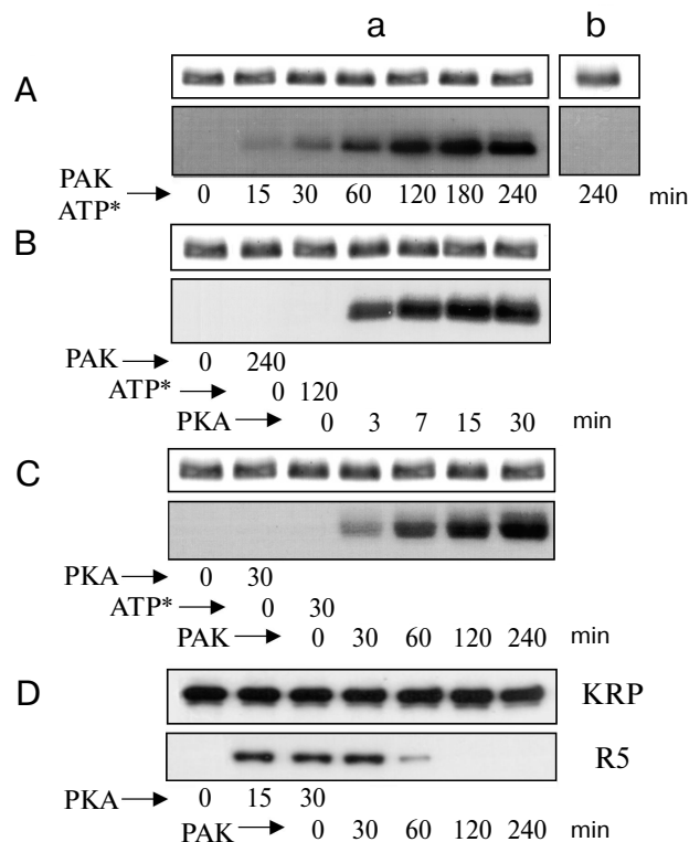
Fig. 3. Phosphorylation of KRP by p21-activated protein kinase PAK1 in vitro and its effect on the R5 antibody binding. Shown is the kinetics of KRP phosphorylation after addition of protein kinase A (PKA) and PAK1 (PAK). ATP* indicates time of the [ \gamma - 32 P]ATP addition. For each experiment, the Coomassie R-250 stained gels and autoradiograms are shown on the upper and lower panels, respectively. A) Phosphorylation of recombinant human (a) and chicken (b) KRP by PAK1; B) sequential phosphorylation of KRP by PAK1 in the absence of [ \gamma - 32 P]ATP and then by PKA added 2 h after the intermediate incubation with [ \gamma - 32 P]ATP to ensure completeness of former phosphorylation with PAK1; C) sequential phosphorylation of KRP by PKA and then by PAK1; the details as in (B); D) KRP was sequentially phosphorylated by PKA and PAK1 as in (C), but in the absence of [ \gamma - 32 P]ATP and analyzed by Western blotting using the R5 antibody against phospho-Ser13 and polyclonal anti-KRP antibody for the load control as indicated.
