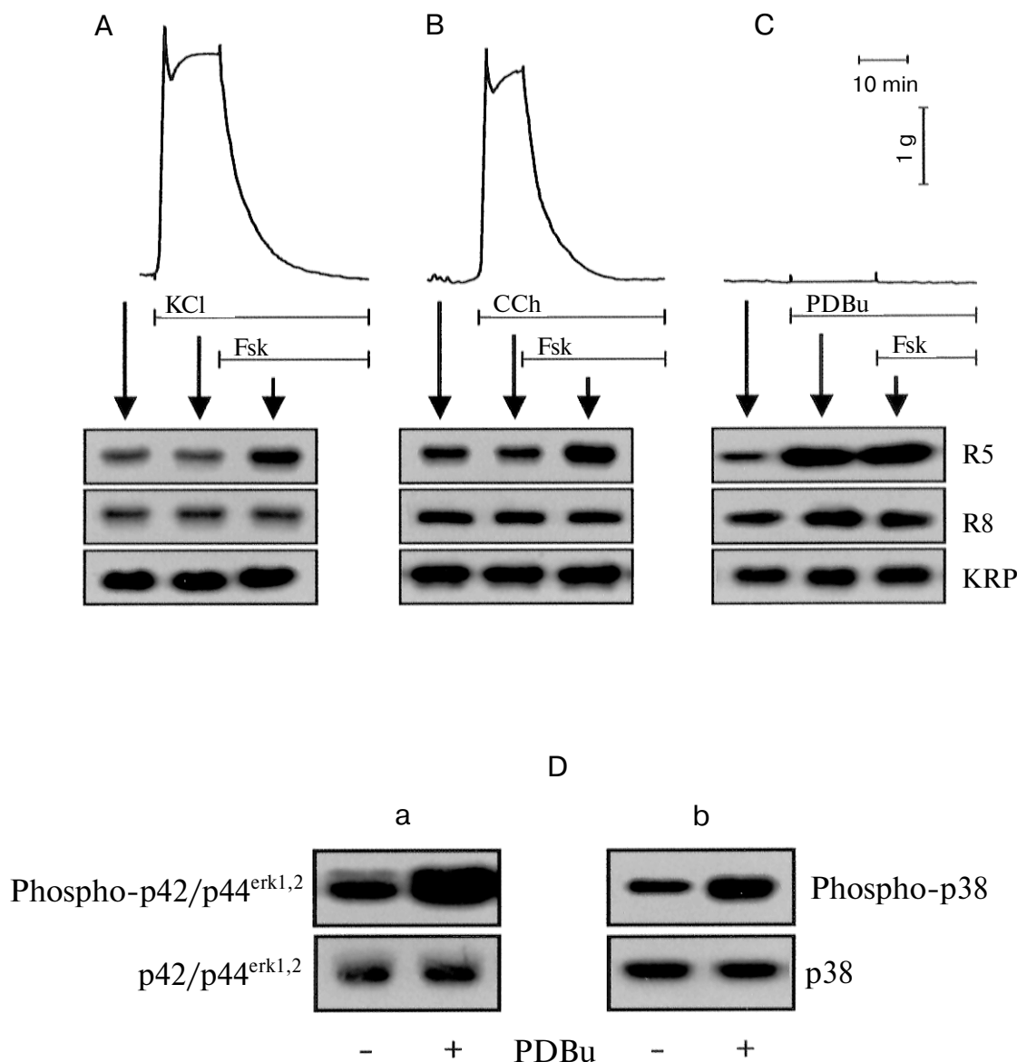
Fig. 6. Phosphorylation of KRP in the smooth muscle contraction–relaxation cycle. The experiments were performed with intact ileum strips as described in the “Materials and Methods” section. The level of KRP phosphorylation was measured in extracts of rapidly frozen tissue using the phospho-specific or polyclonal antibodies. Shown are typical immunoblots from three independent experiments. A) Mechanograms of rat ileum contraction induced by membrane depolarization with 90 mM KCl. After contraction had reached a plateau, the relaxation was stimulated by adding forskolin to 10 \mu M (Fsk). Phosphorylation of KRP at Ser13 (R5) and Ser19 (R8) and its total amount (KRP) were determined by Western blots at the time points indicated by arrows; B) as in (A), contraction was stimulated by 20 \mu M carbachol (CCh); C) as in (A), the muscle was stimulated with 1 \mu M PDBu. Note that PDBu does not evoke contraction in phasic smooth muscle [23]; D) 1 \mu M PDBu activates both p42/44 erk1,2 (a) and p38 (b) MAP-kinases in intact ileum. MAP-kinase activation was measured with phospho-specific (upper panels) and polyclonal (lower panels) antibodies against MAP-kinases as described in “Materials and Methods”.
