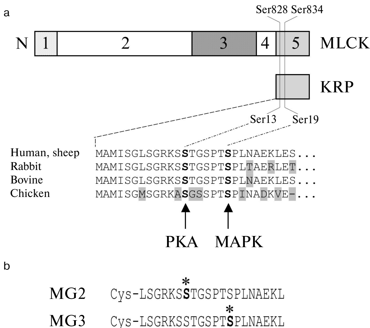
Fig. 1. Domain organization of MLCK and KRP and sequences of synthetic peptides used for production of phosphospecific antibodies. a) Domain organization of MLCK and KRP. Shown are the relative positions of the N-terminal actin-binding domain (1), tandem repeats (2), catalytic domain (3), regulatory calmodulin-binding segment (4), and the myosin-binding domain of MLCK that is separately expressed in smooth muscle as KRP (5). The N-terminal sequence of KRP from different species is zoomed underneath. The numbering of common MLCK and KRP sites phosphorylated by protein kinase A (PKA) and MAP-kinase (MAPK) is according to chicken proteins (see [5] for details). b) Sequences of phosphopeptides used for immunization. Asterisks denote position of residues with associated phosphate group.
