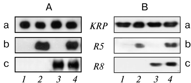
Fig. 2. Phospho- and site-specificity of the R5 and R8 antibodies. Recombinant human (A) and chicken (B) KRP (40 ng in each lane) was fully phosphorylated by PKA (2), p44 erk1 -MAP-kinase (3), or both kinases (4). Lane 1 contains unphosphorylated KRP. The Western blot was probed with polyclonal antibody against KRP (a) and phospho-specific antibody against Ser13 (R5 (b)) or Ser19 (R8 (c)).
